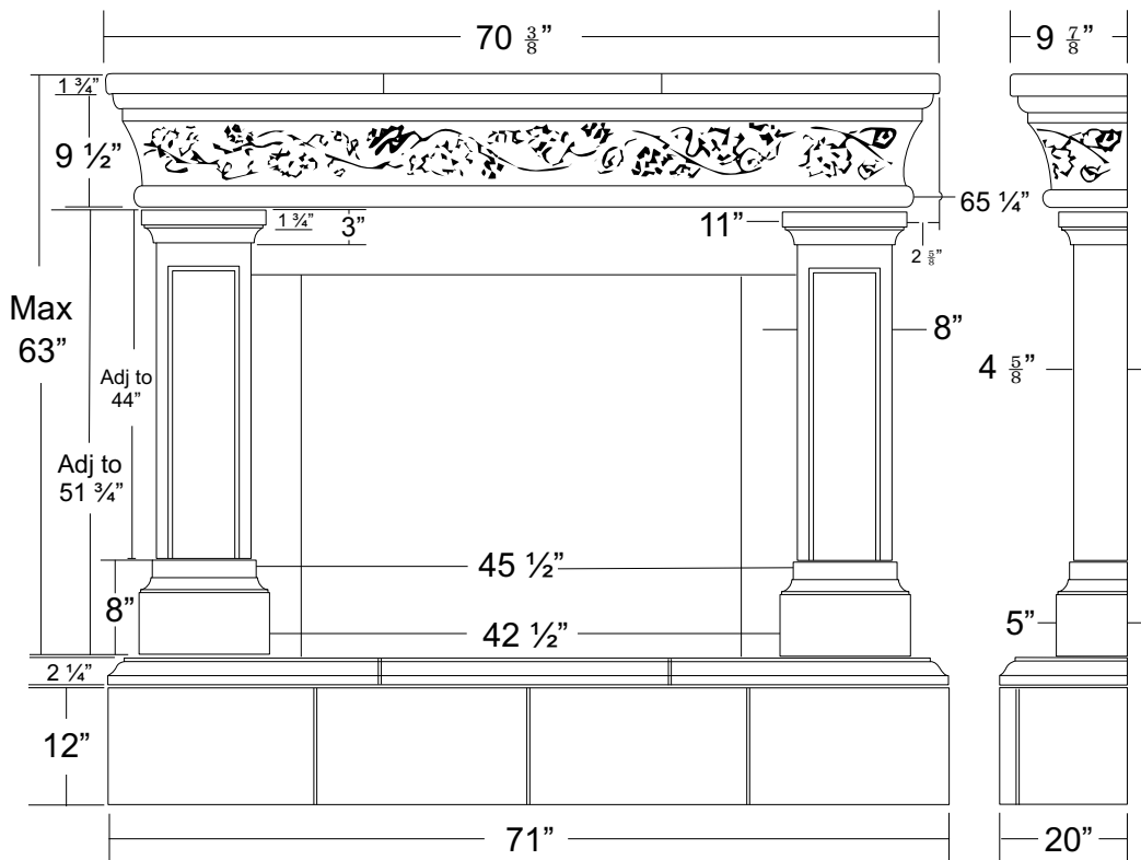
FS142 - Multi Piece
